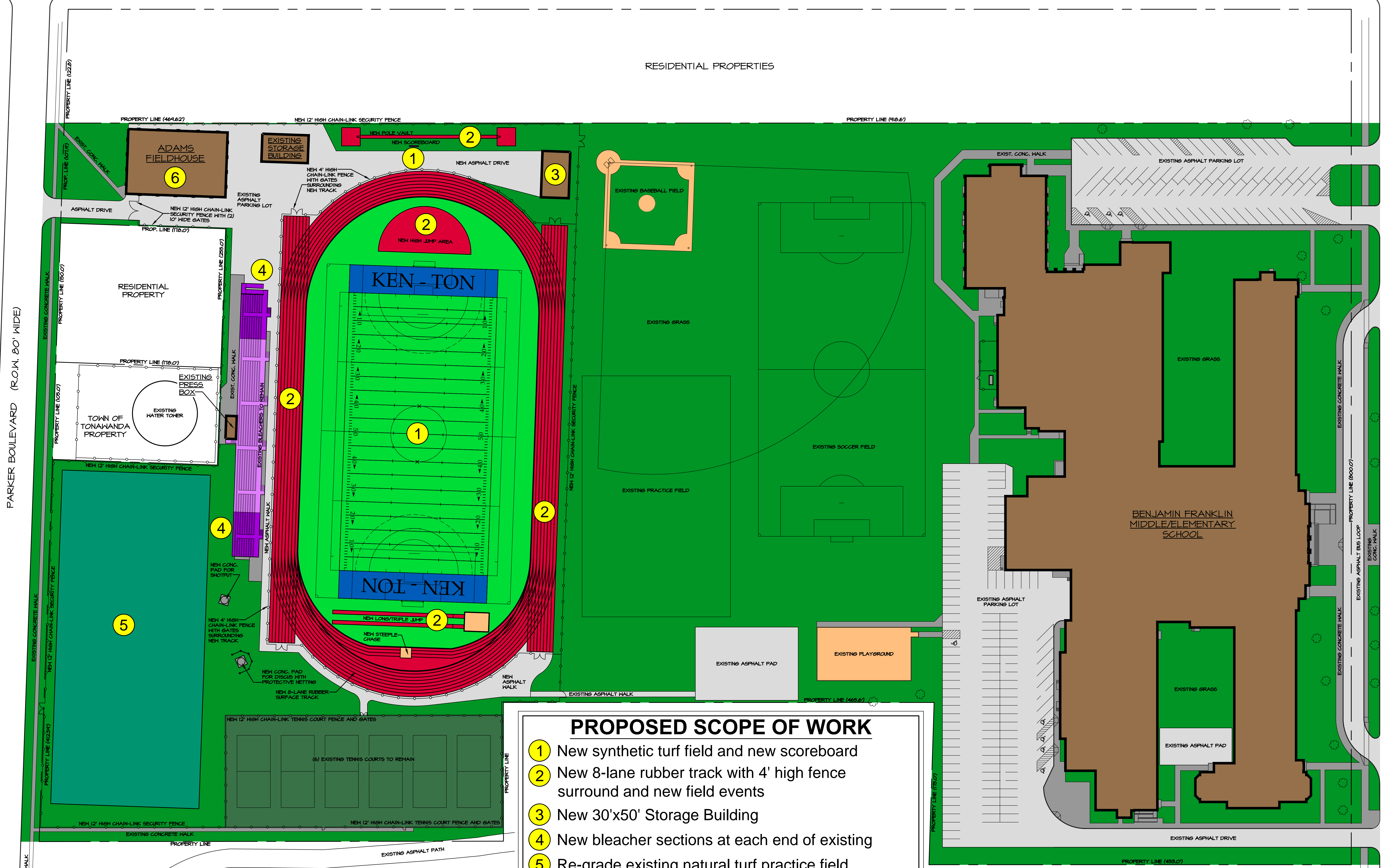
ADAMS FIELD OVERALL SITE PLAN
